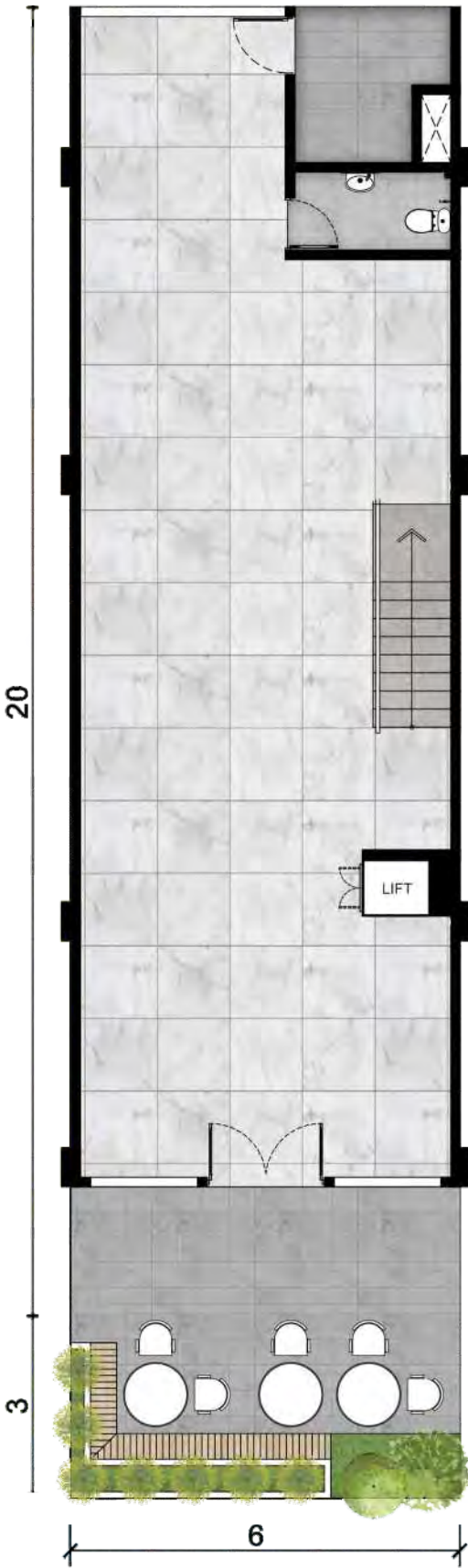
1 st FLOOR PLAN
