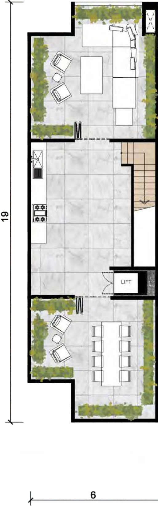
ROOFTOP PLAN
