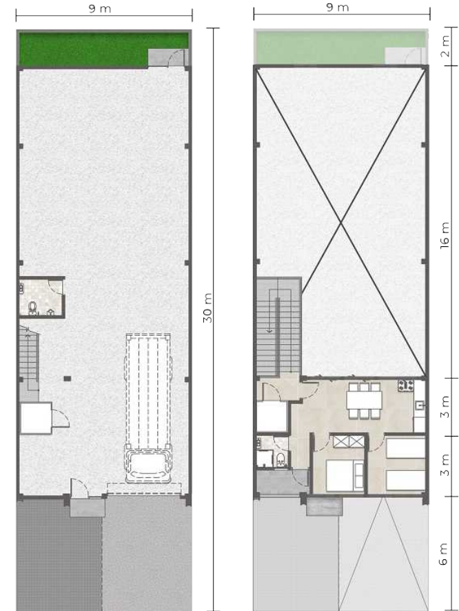
DENAH LT.2
